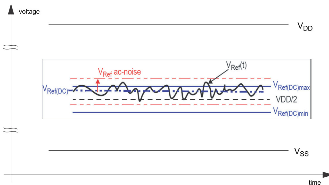
V_{REF}(DC) tolerance and V_{REF} AC-Noise limits
