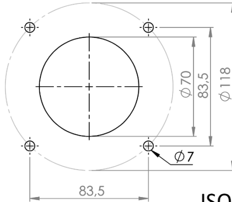
Mounting Cut-Out Enclosure Ø130 mm
