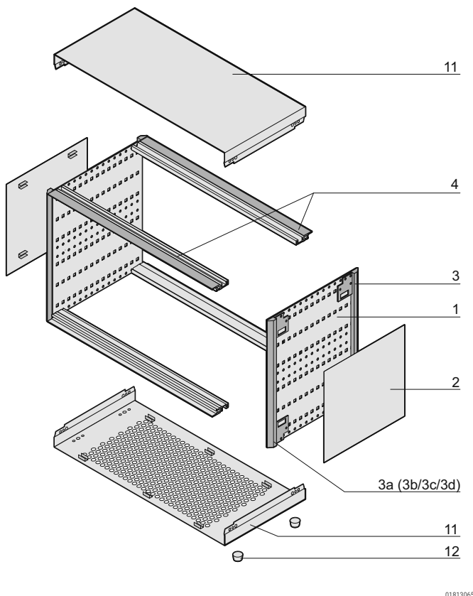
Drawing with front cover strip
