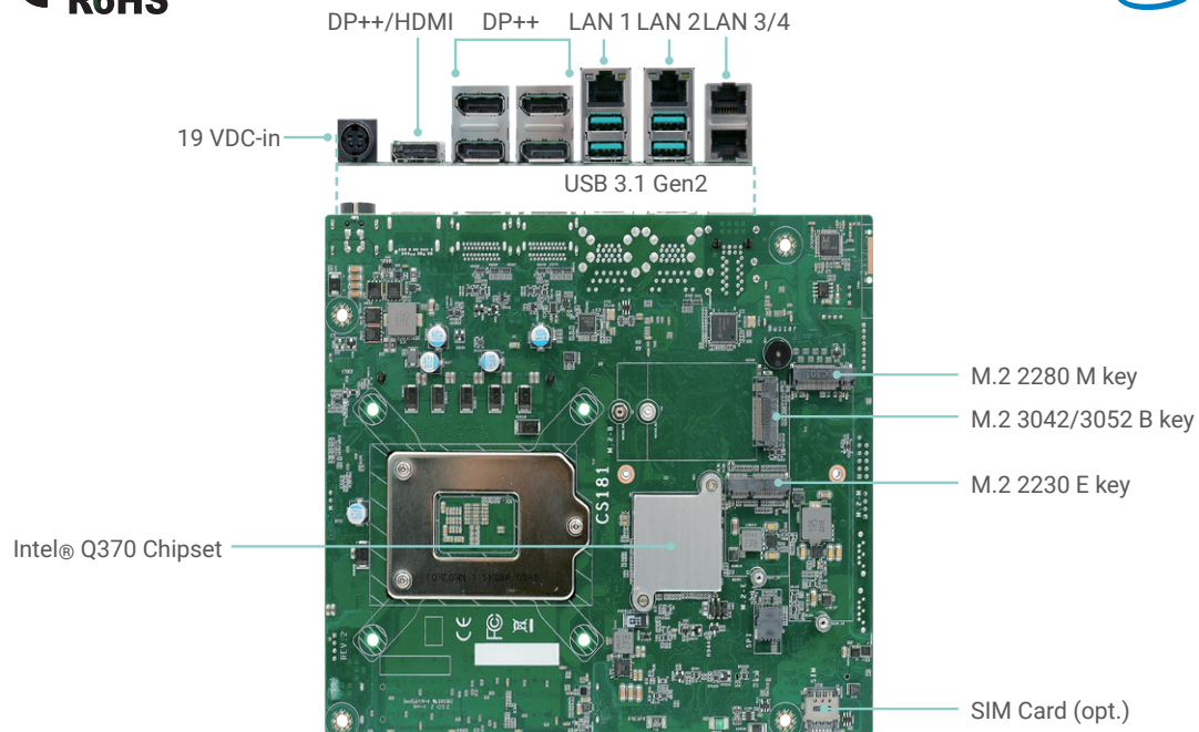
Bottom View
