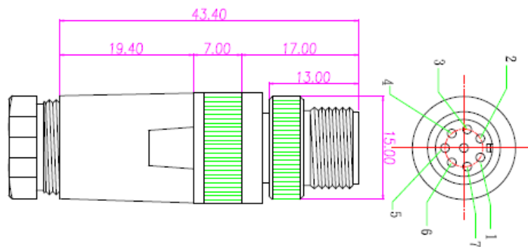
M12P-8MA dimension (mm)
