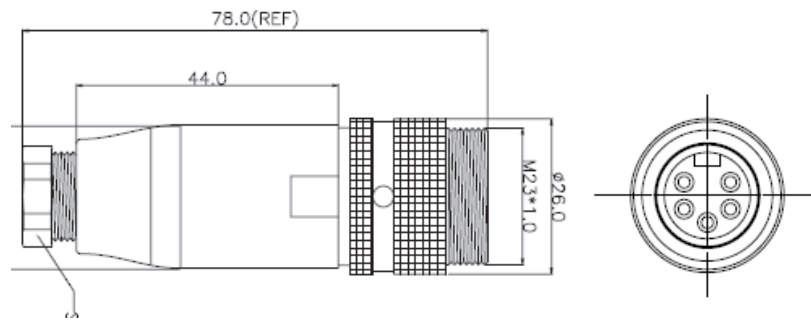
M23P-5MA dimension (mm)
