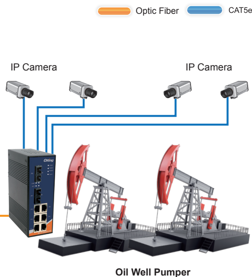
Connections of Ethernet devices
