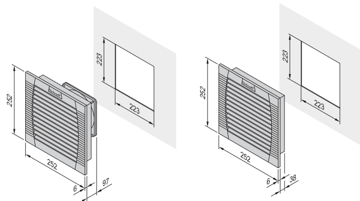
Air filtered fan FL 250 Air outlet/inlet filter FLA 250/300 Sheet thicknesses 1 ... 2 mm - cut-out 223 x 223 mm; Sheet thicknesses >2 ... 3 mm - cut-out 224 x 224 mm
