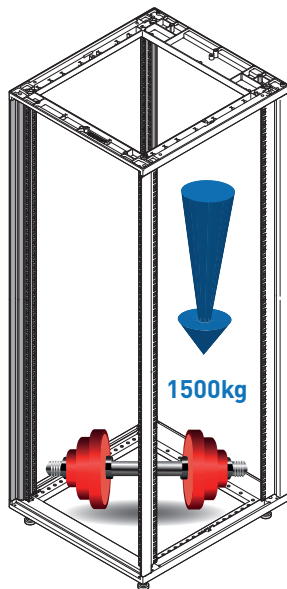
Vertical static load
