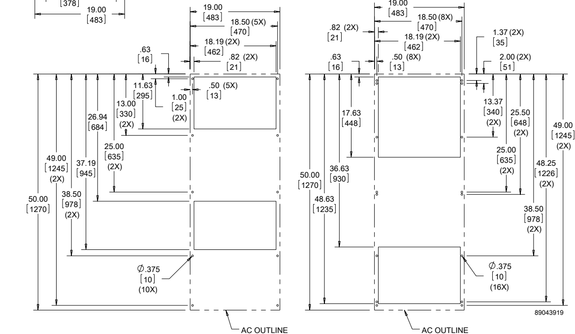
Cutout Dimensions (Externally Mounted)
