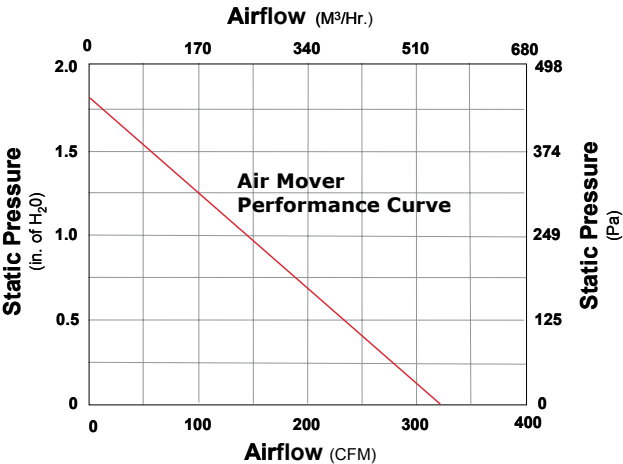
Air Mover Performance Curve Example
