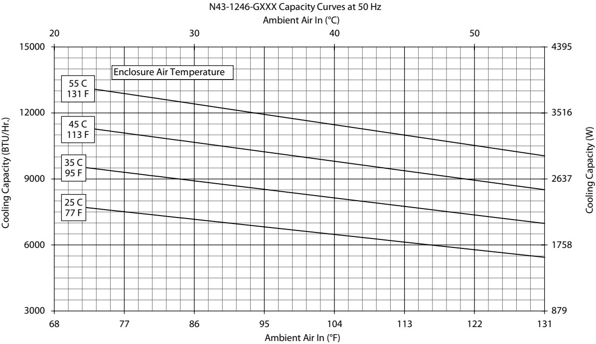
Performance Curves for N43 Models 11000 BTU/Hr. (3223 Watt)
