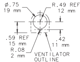
Small Ventilator
