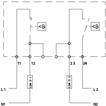
CONNECTION DIAGRAM
