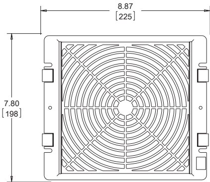
TEP6 EXHAUST GRILLE
