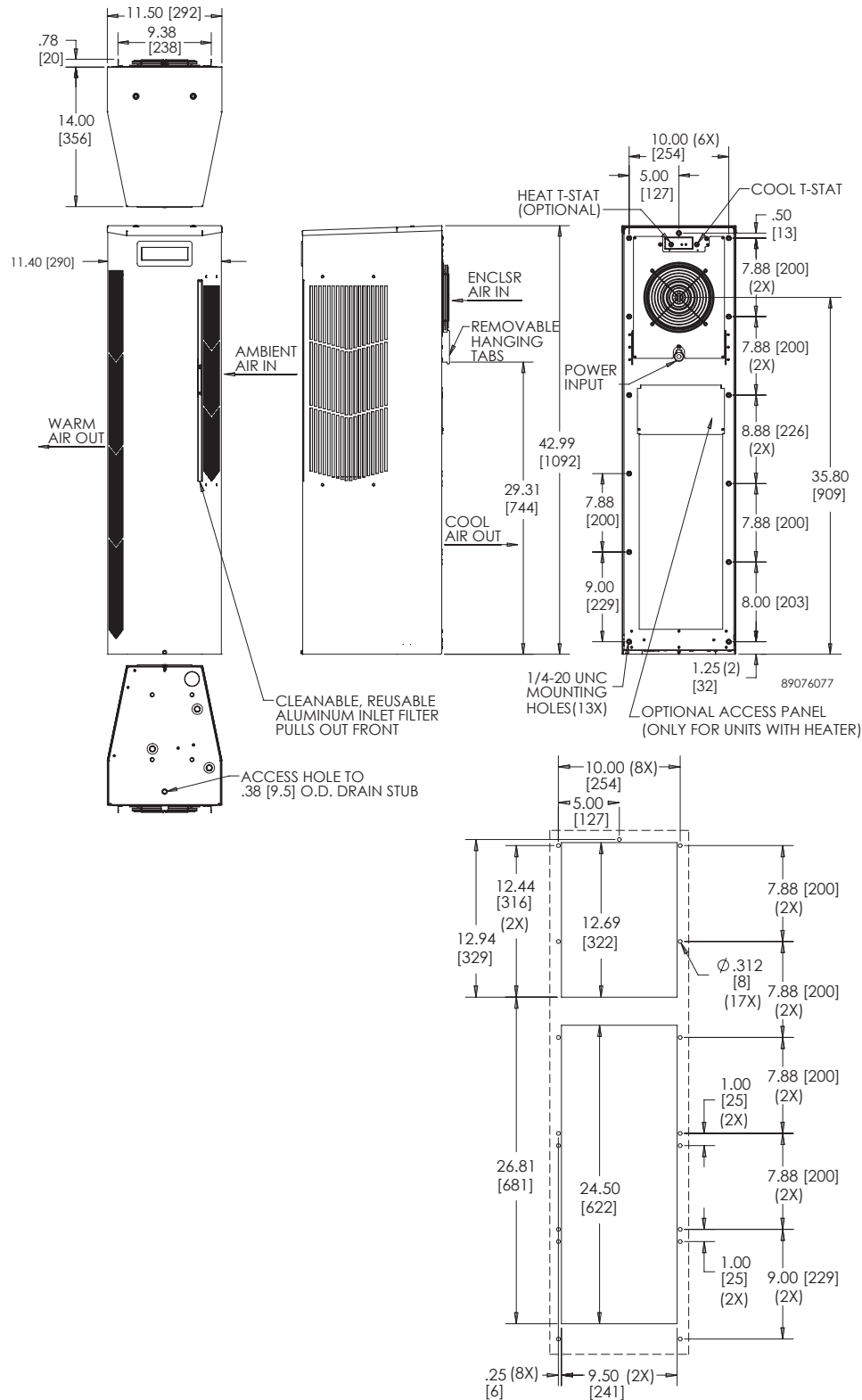
CUTOUT INSTRUCTIONS
