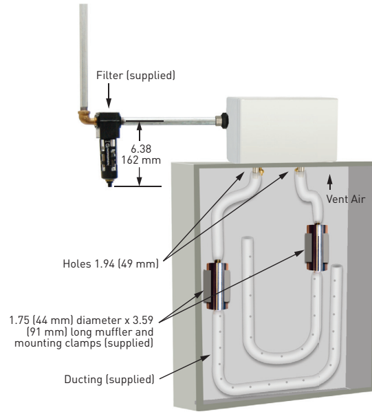
VA50, Type 4/4X
