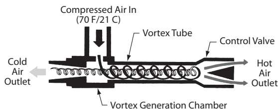
Vortex Tube Air Flow Schematic
