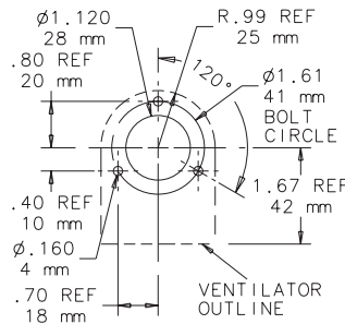
Large Ventilator
