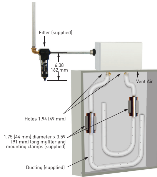
VA50, Type 12
