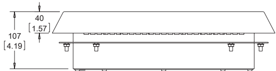
Filter Fan SR16 459 CFM (780 m³/hr)
