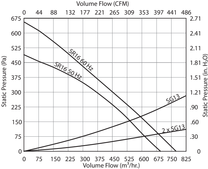
SR16 459 CFM (780 m³/hr.) Roof-Mount Filter Fan Performance Curve
